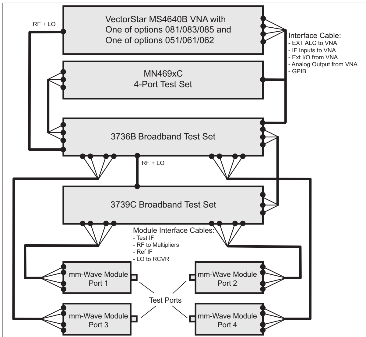
ME7838G4 4-Port Millimeter-Wave Configuration Block Diagram
